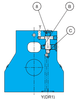
Cross-sectional R-R
