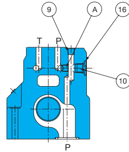
Cross-sectional P-P
